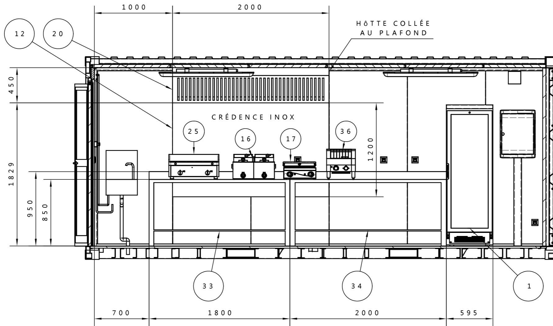
C - C (1:30)
