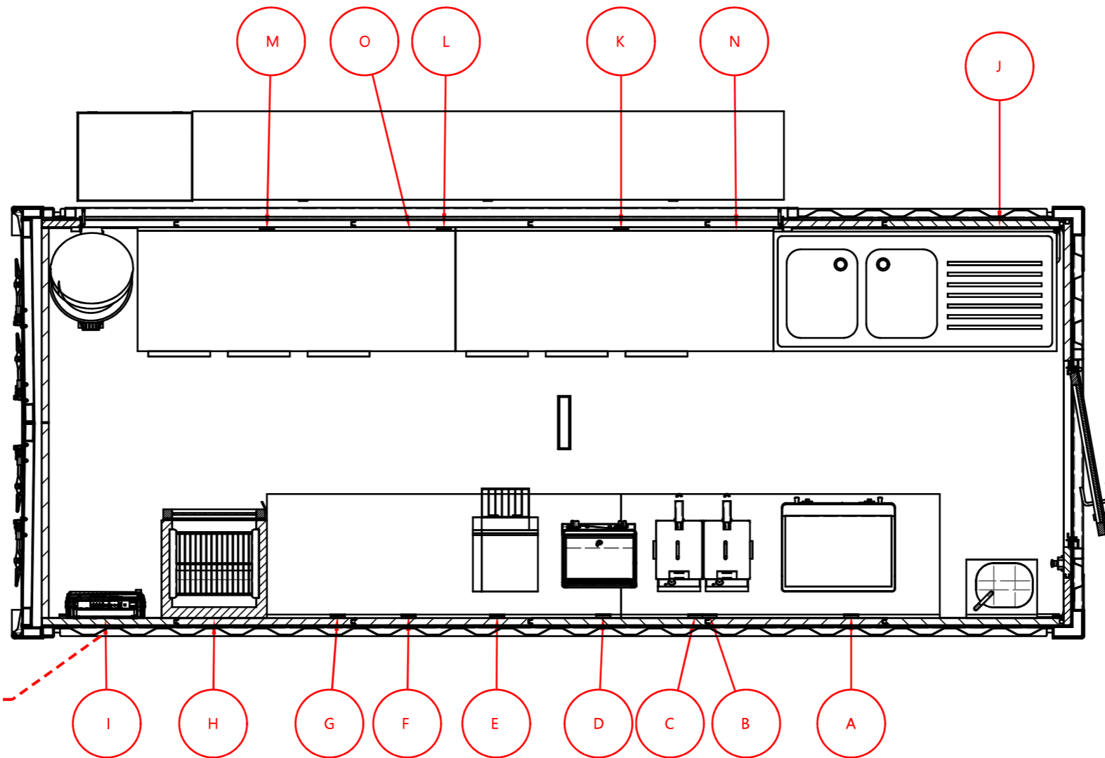
B - B (1:30)
